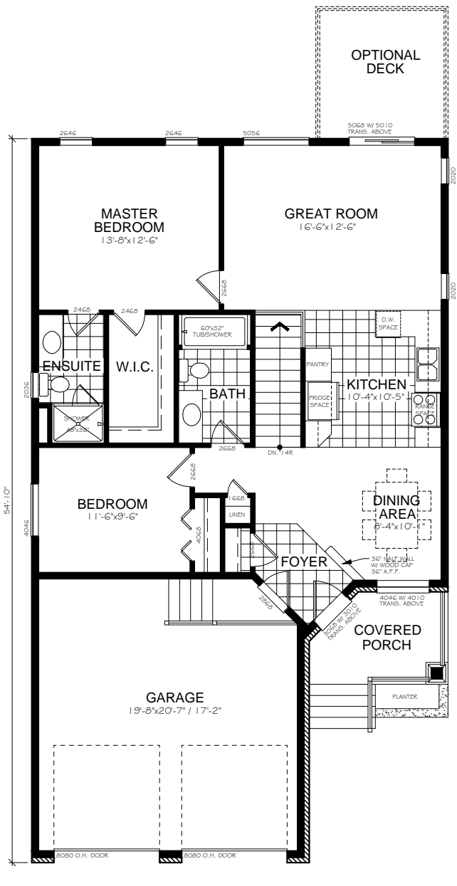
OPTIONAL MAIN FLOOR PLAN
