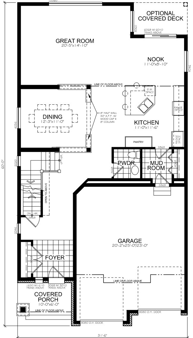
MAIN FLOOR PLAN FLOOR AREA=1195 SQ.FT.
