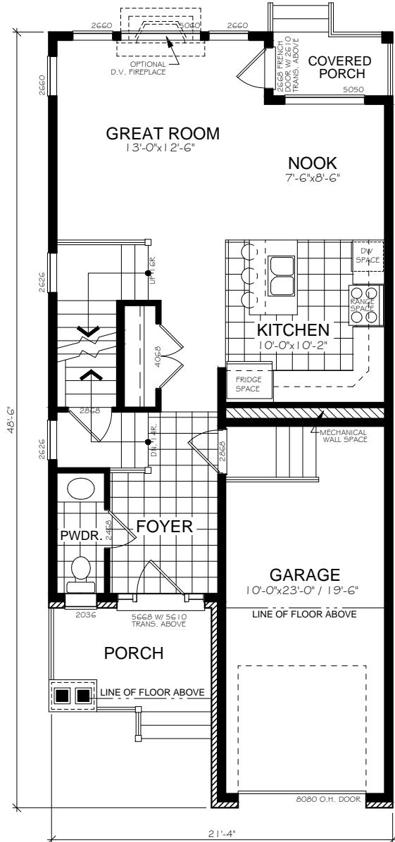
MAIN FLOOR PLAN 615 SQ.FT.
