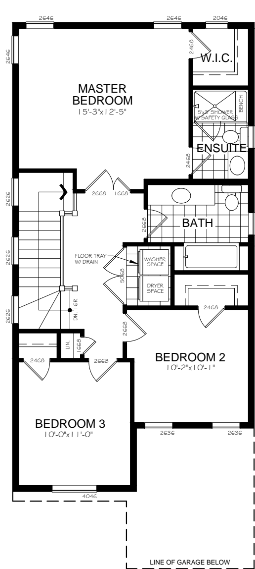
UPPER FLOOR PLAN 770 SQ.FT.
